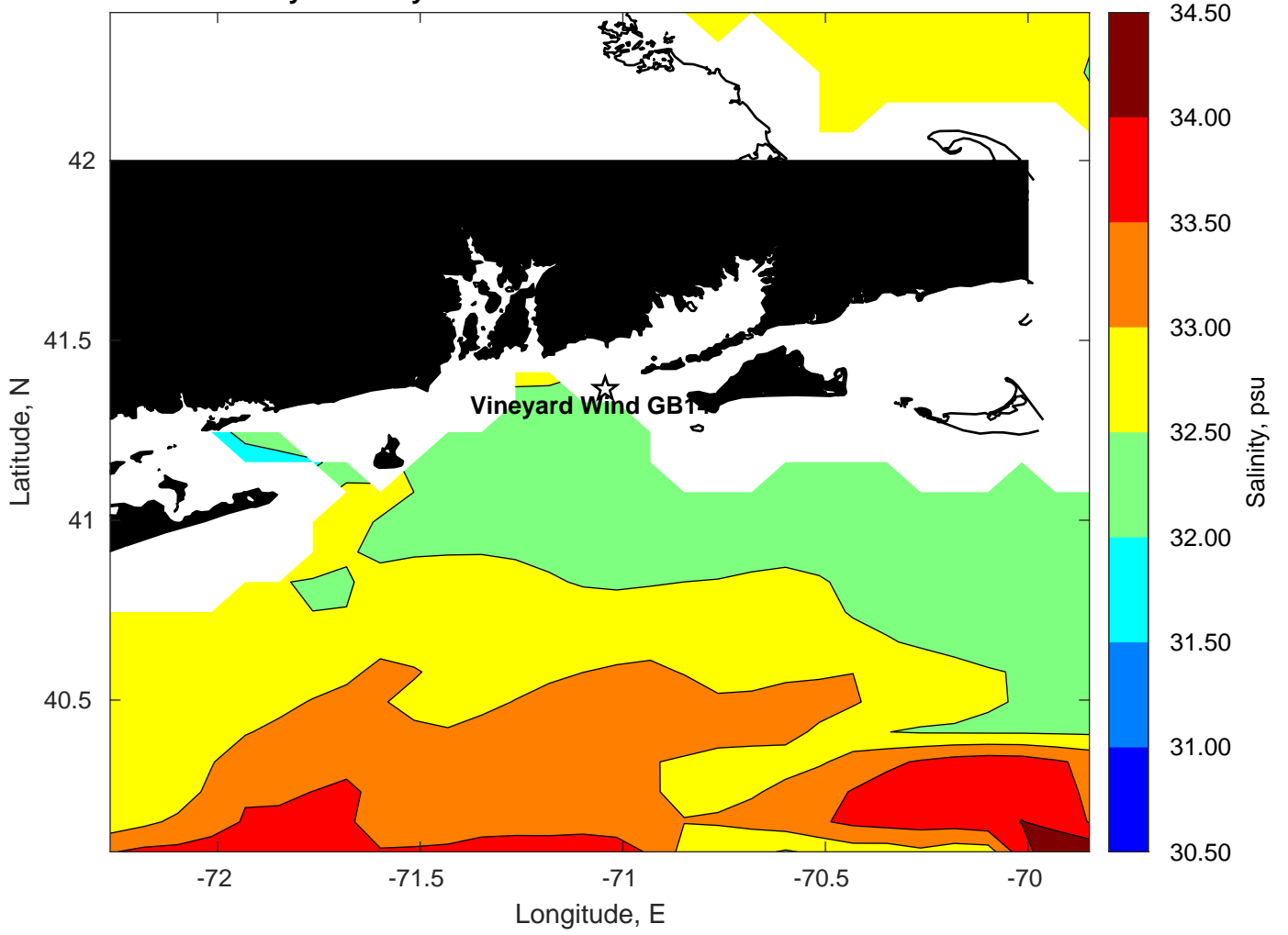
Surface Salinity for Vineyard Wind GB14 at 13-Oct-2022 00:00:00
